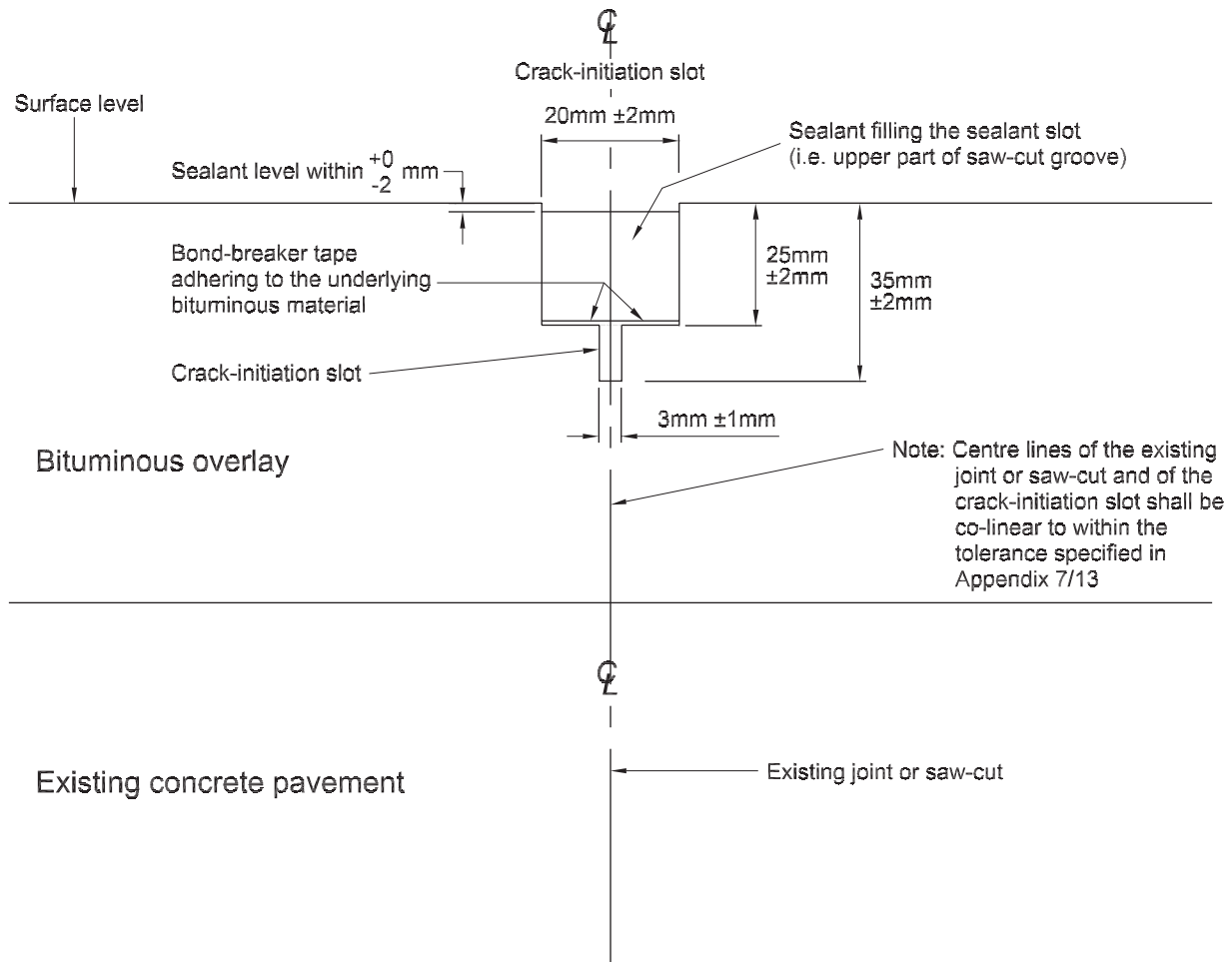
FIGURE 7/1: (02/16) Detail of Saw-cut and Seal Groove with Sealant in Bituminous Overlay
