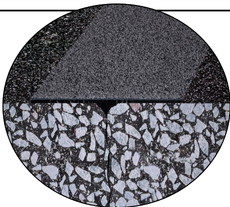
Transverse & Longitudinal repairs
